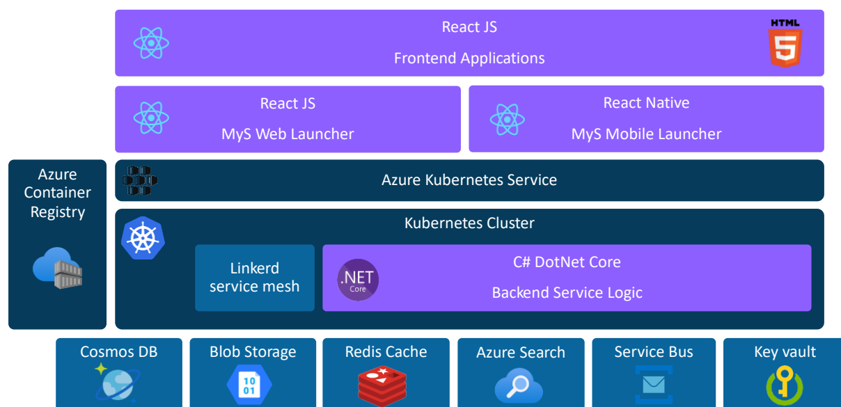
Figure 2: Layered infrastructure architecture based on microservices and extensive use of managed services provided by the Azure cloud environment.
